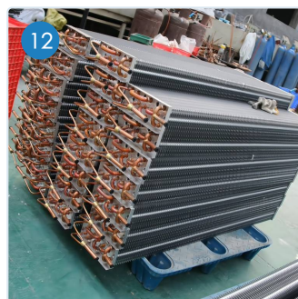
大型蒸发器成品 Large Evaporator Finished
