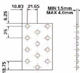
6 \Phi 6.0*25*21.65(2) FLAT (LOUVER)
