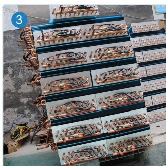
多排冷凝盘管 Multi-row Condenser Coils
