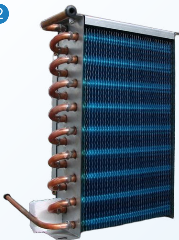
铜管铝翅片蒸发器 Copper-tube Aluminum-fin Evaporator
