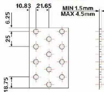
2 \Phi 7.0*25*21.65(2) FLAT (LOUVER)
