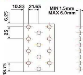
5 \Phi 6.0*25*21.65(1) FLAT+WAVE (CORRU6A TED)
