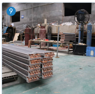
立式冷柜蒸发器板 Upright Evaporator Panels
