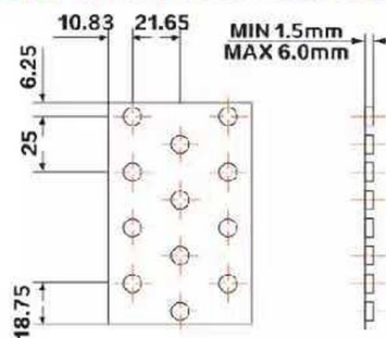
1 \Phi 7.0*25*21.65(1) FLAT+WAVE (CORRU6A TED)
