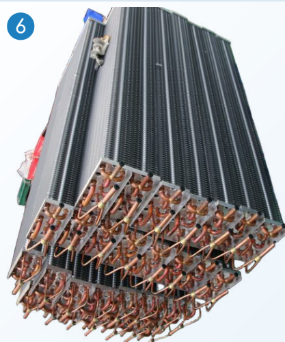
糖葫芦蒸发器芯体 Tanghulu-type Evaporator Core
